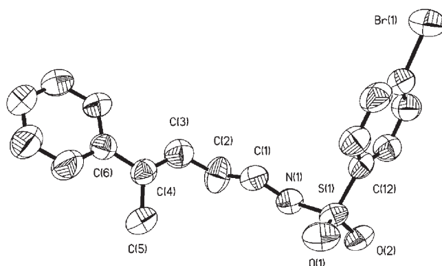
Figure 1. ORTEP representation of compound E - 2ab (probability ellipsoids at the 50 % level). Selected bond lengths (Å) and angles (°): S(1)–N(1), 1.609(4); N(1)–C(1), 1.472(6); C(3)–C(4), 1.320(7); C(1)–N(1)–S(1), 120.7(3).
