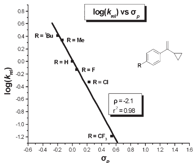
Figure 2. Hammett plot for the ring-opening of 1a–f with TsNHMe using PPh 3 /AuOTf as catalyst.
