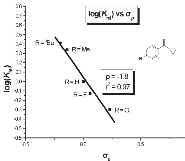
Figure 3. Hammett plot for the ring-opening of 1a–e with TsNHMe using HOTf as catalyst.
