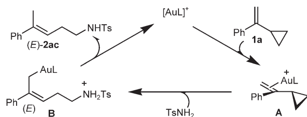
Scheme 2. Plausible simplified reaction mechanism for the Au(I)-catalyzed ring-opening of VCP 1a .
