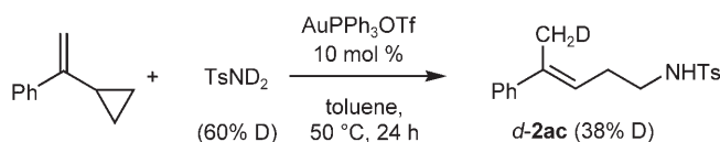
Scheme 1. Deuterium labelling experiment.
